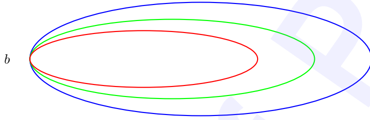
FIGURE 1. The pencil \mathcal{P}_1
