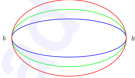
FIGURE 2. The pencil \mathcal{P}_2
